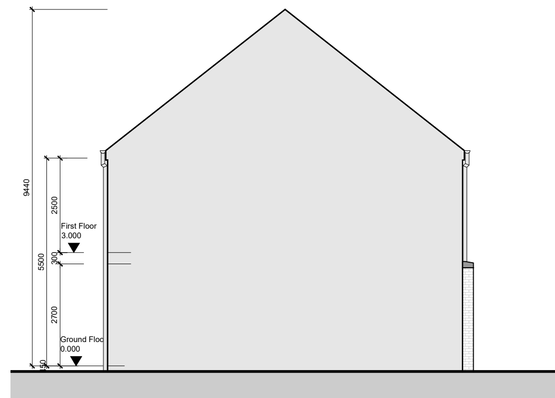
Side Elevation 01
